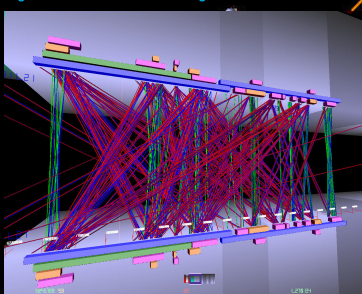
Fig. 3: Intra-chromosomal duplicons (Eichler et al.) compared to syndromes (blue/green), literature hot-spots (orange), and our defined hot-spots (pink) of the chr. 22q.11 region.
