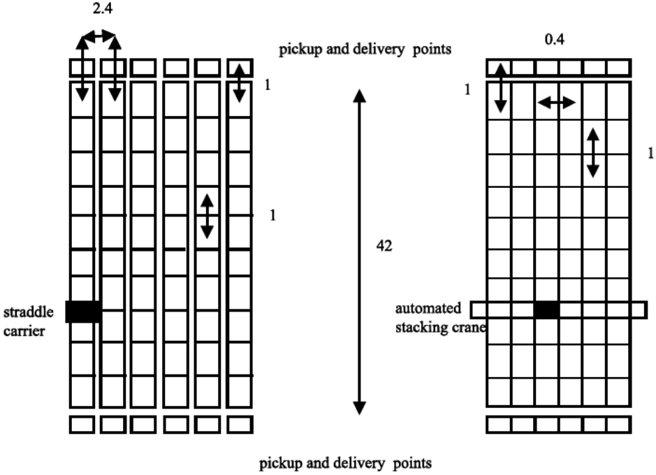
FIGURE 9.3. Illustration of distances in stack used in this simulation study.
