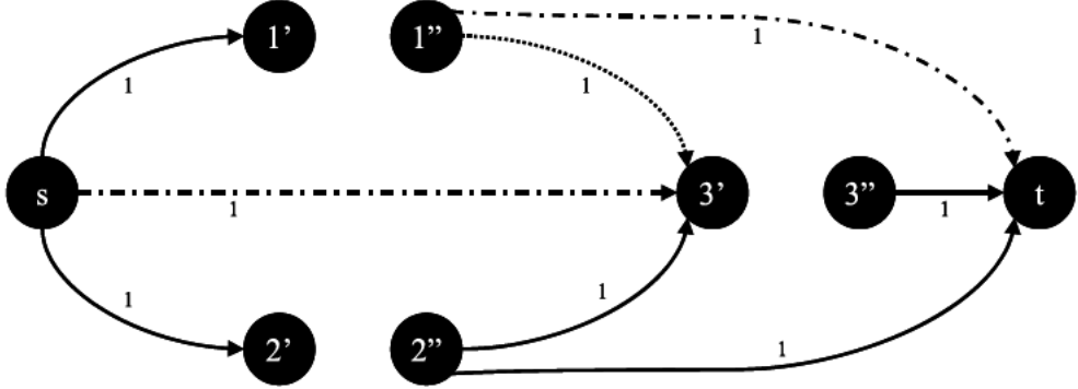
FIGURE 3.3. Graph G_2 with forward arcs (-.-) and backward arcs (\dots) that belong to the maximum flow.
